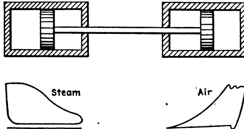
FIG. 47.—Direct acting steam compressor.
